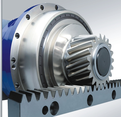
RACK & PINION
